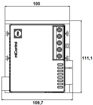
Mounting / Heat sink drawing
