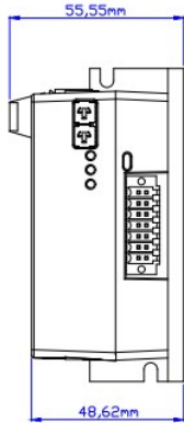
Mounting / Heat sink drawing
